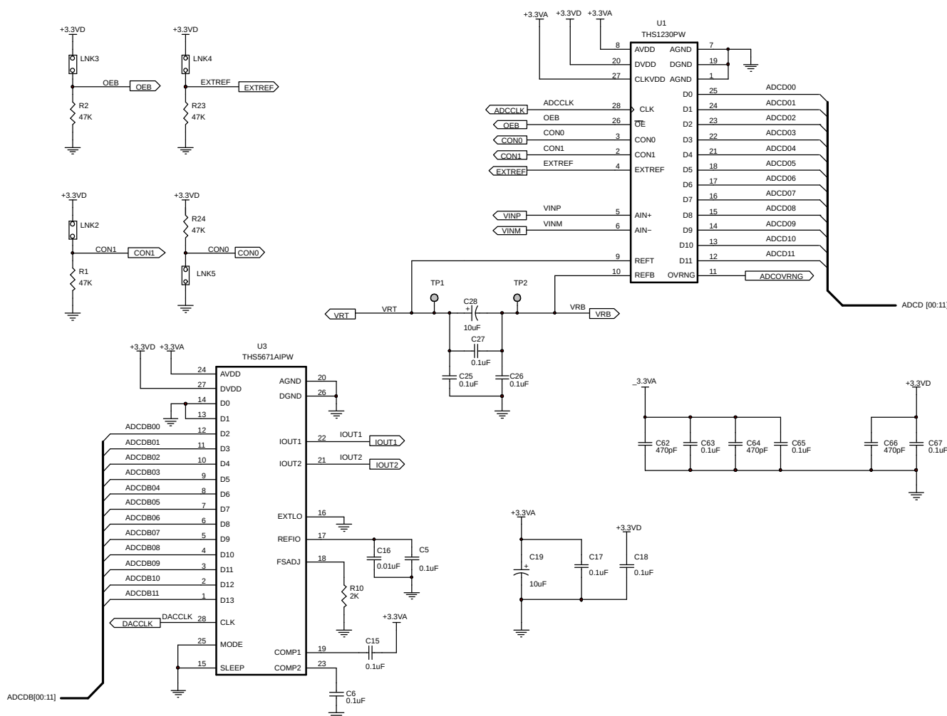
Figure 22. EVM Schematic
